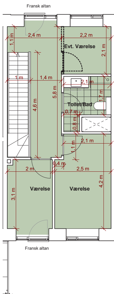
1 sal
